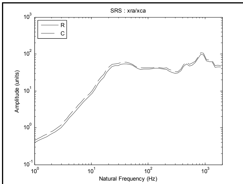
Figure 525A-24b. Composite pseudo-velocity maximax acceleration SRS for r and c.
