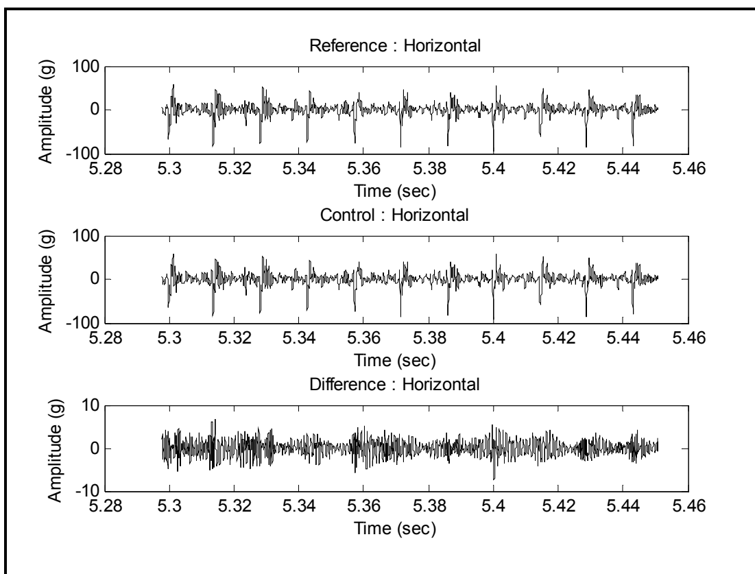
Figure 519.6A-5. High resolution representative members for the pulse ensembles (4000 round/minute).
