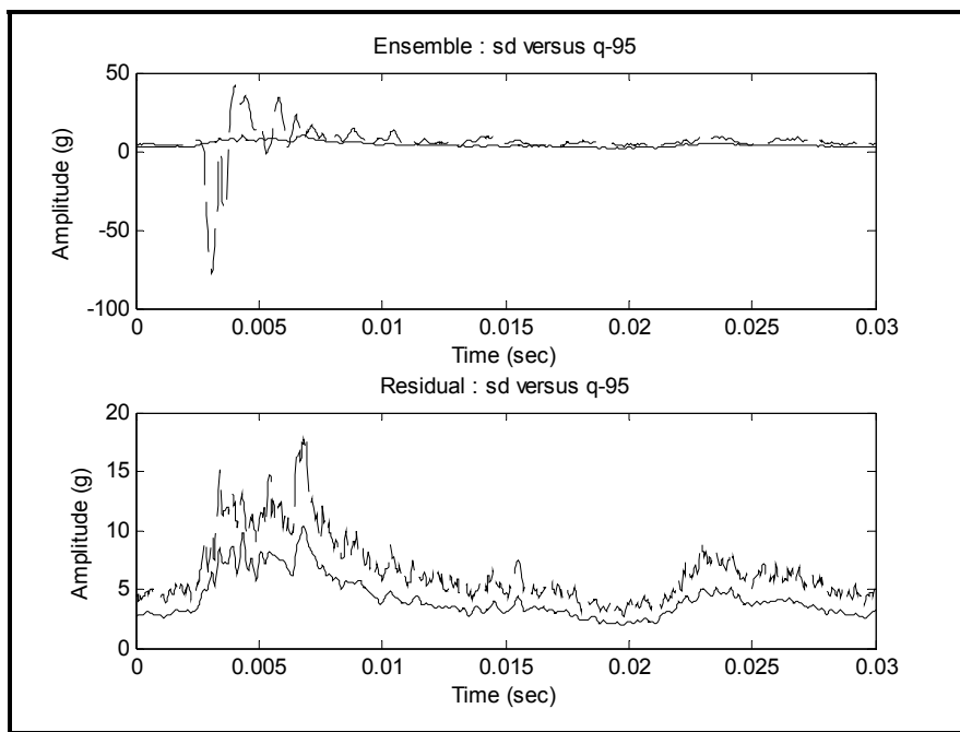
Figure 519.6E-3a. Time-varying standard deviation versus the 95 th quantile to time-varying standard deviation.
