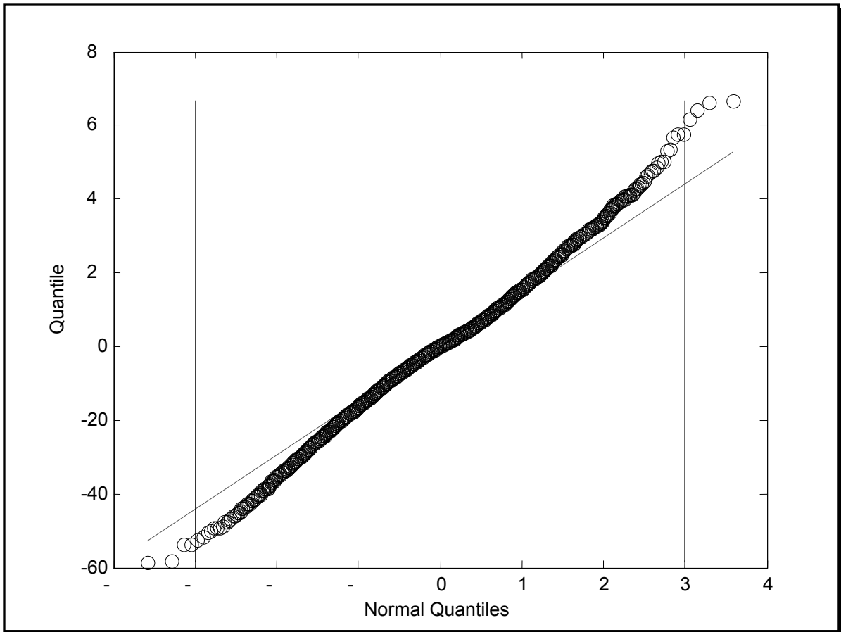
Figure 519.6B-7b. qq-Plot for composite random component decomposition 4000 rnd/min.
