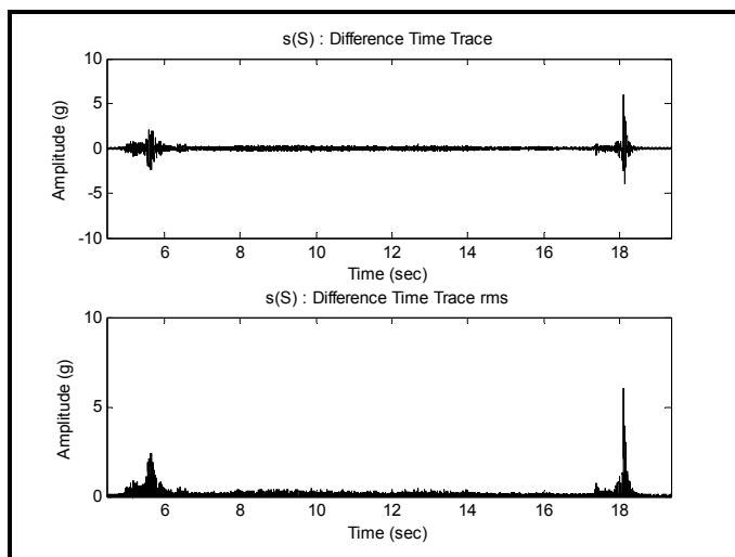
Figure 525A-9b. Difference Exciter (S).
