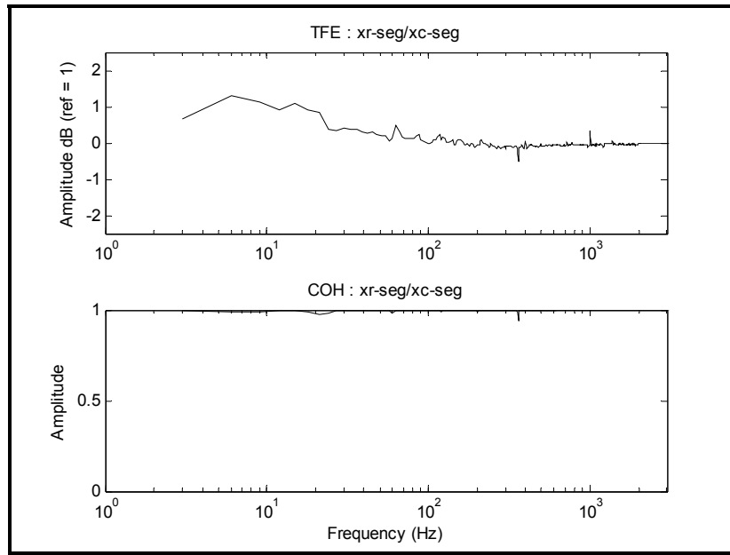
Figure 525A-19. SISO estimates - input r and output c .
