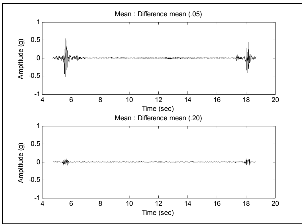
Figure 525A-27. Short-time averaging for difference mean.
