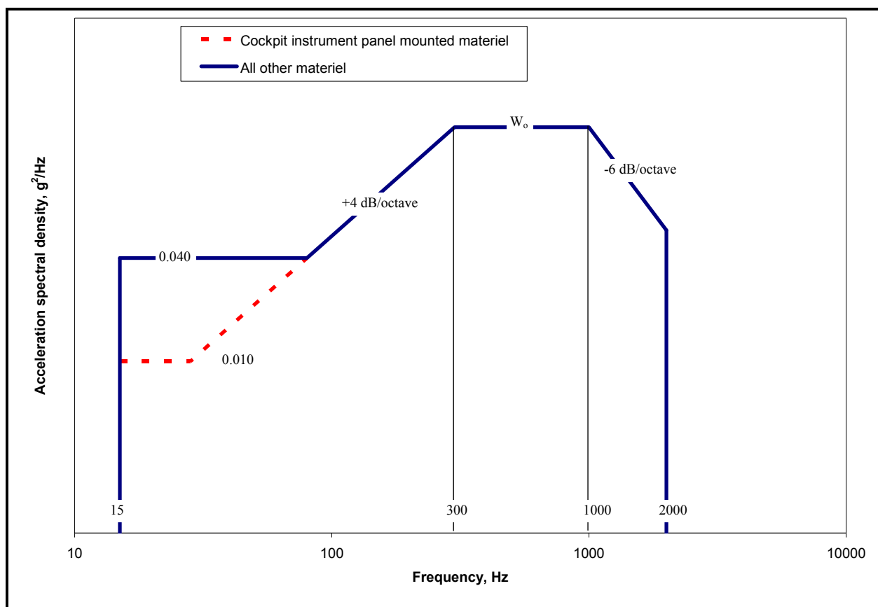
Figure 514.6D-1 - Category 12 - Fixed wing aircraft - jet aircraft. (Same as Annex C, Figure 514.6C-6.)
